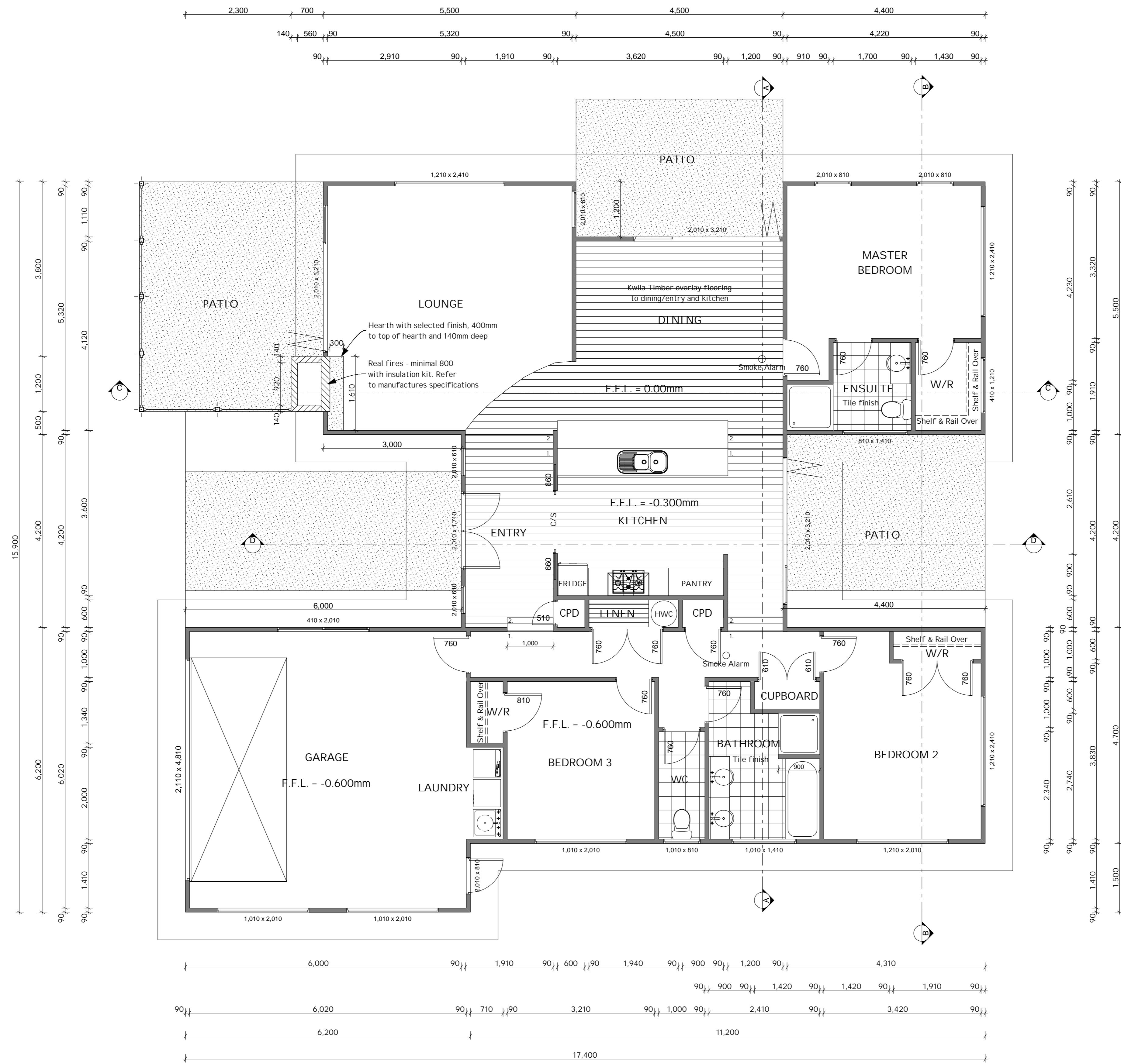
FLOOR PLAN
