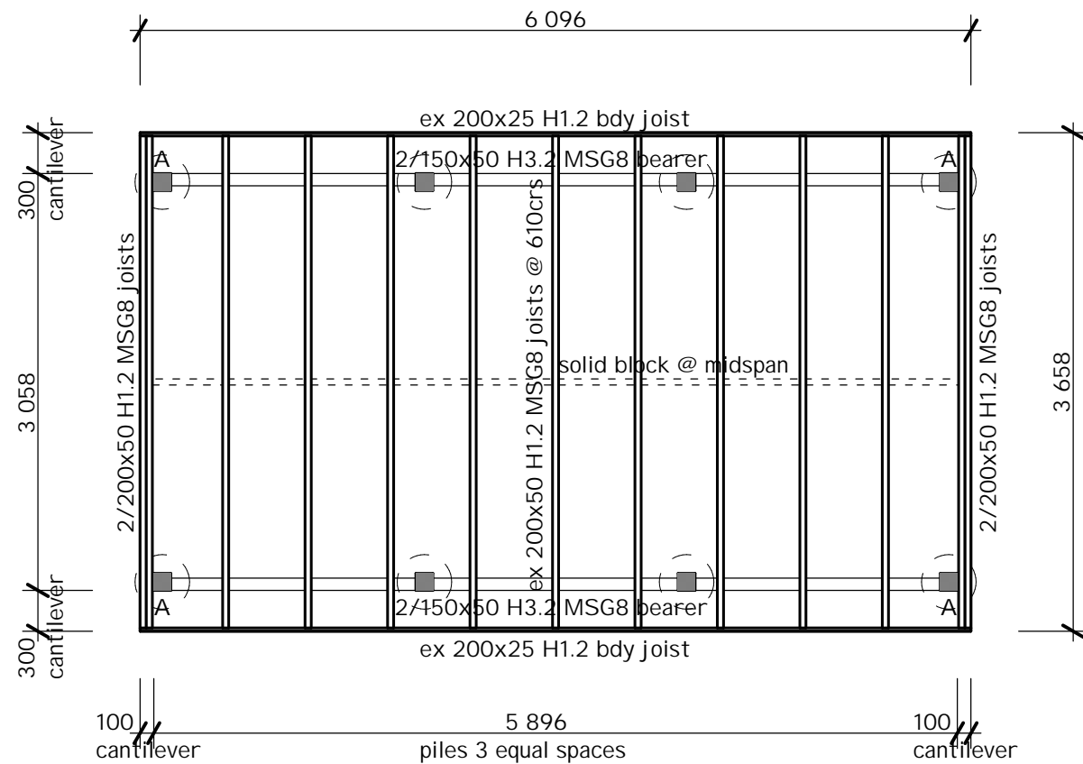
FLOOR FRAMING PLAN
